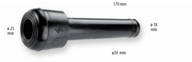
adapt. 23178-01
