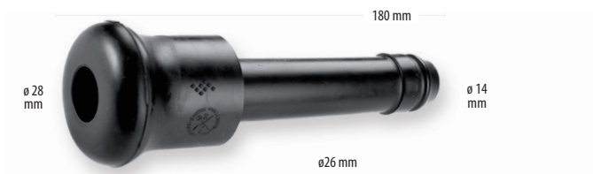
adapt. 68278
